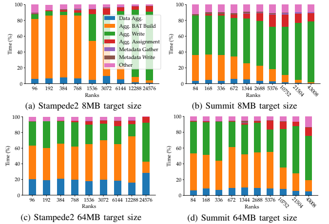
Fig. 6: Timing breakdowns on Stampede2 and Summit. In the scaling regime of each target size, the relative time spent in each component remains similar.
