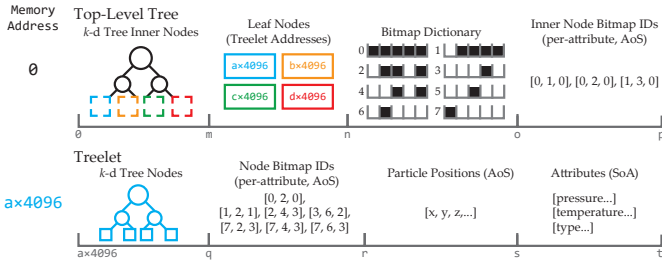
Fig. 2: The BAT layout is organized on disk for fast spatial and attribute query traversal and LOD via memory mapping. The top-level tree is stored at the start of the file in two parts. The first section contains the k -d tree inner nodes, followed by the leaf nodes. The leaf nodes are addresses of the corresponding treelet in the file. The shared bitmap dictionary is also stored at the start of the file, along with the IDs of the top-level tree’s inner node bitmaps. Each treelet is aligned to a 4KB page boundary for fast access via memory mapping. Each treelet consists of the k -d tree and the bitmap IDs for each node, followed by the particle data.
